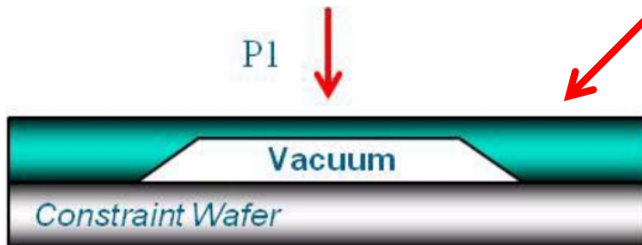
Cross section of absolute pressure-sensing element
